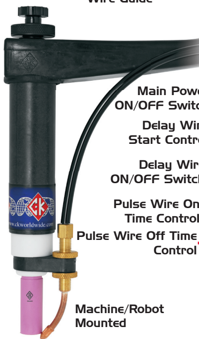
Head Mounted Wire Guide
